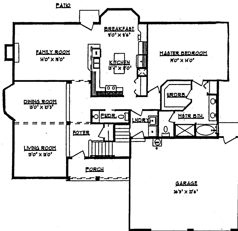
Main Level
